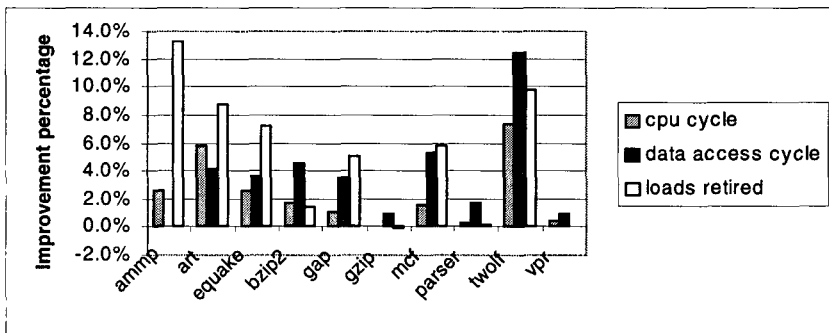
Figure 8. Performance of speculative register promotion
