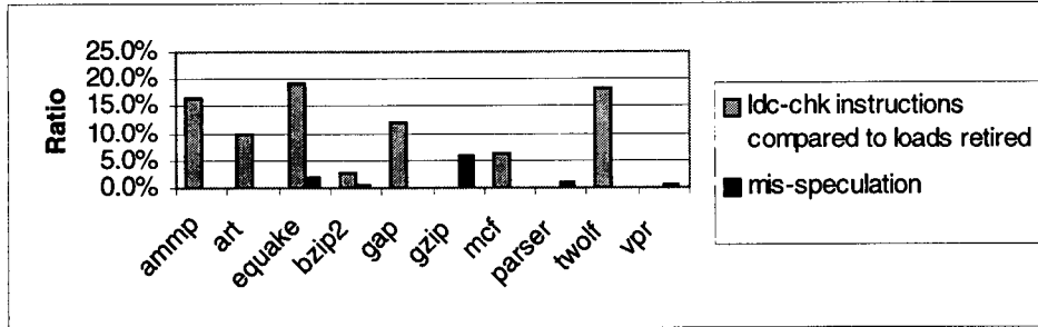
Figure 10. The mis-speculation in speculative register promotion
