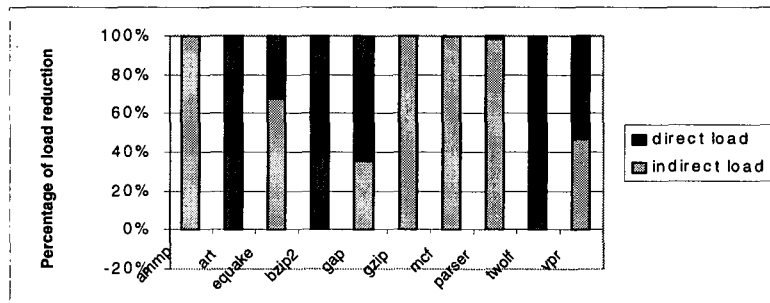
Figure 9. Percentage of different types of load among total reduced load
