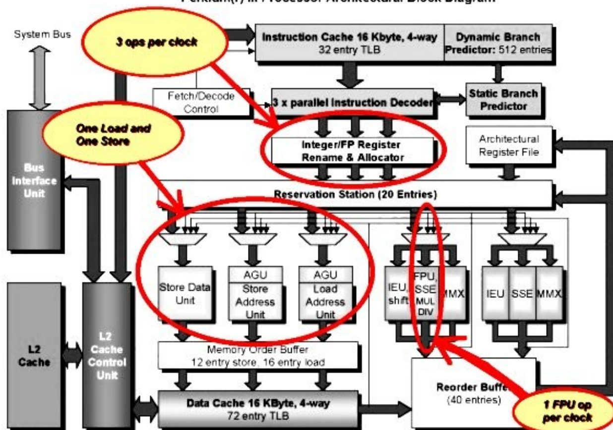
Pentium(r) III Processor Architectural Block Diagram
