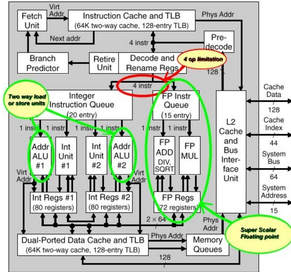
The Compaq Alpha 21264
