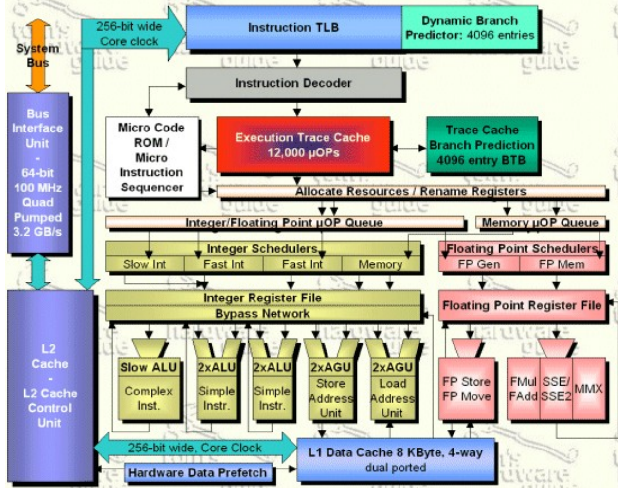
Pentium(r) 4 Processor Architectural Block Diagram
