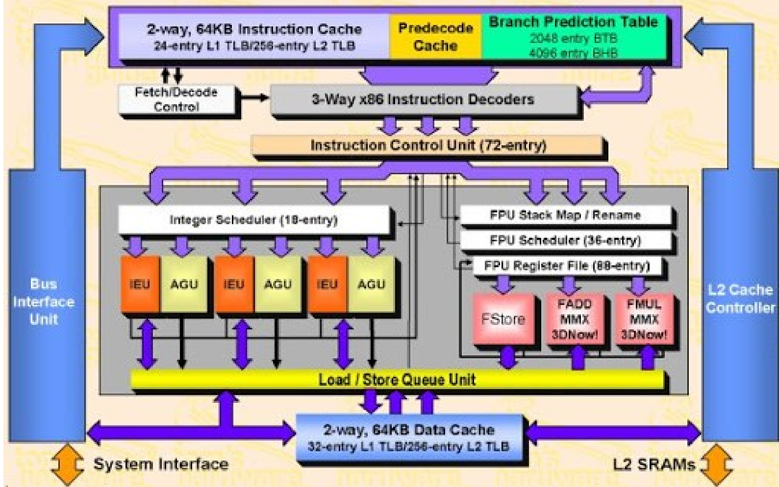
AMD Athlon™ Processor Architectural Block Diagram
